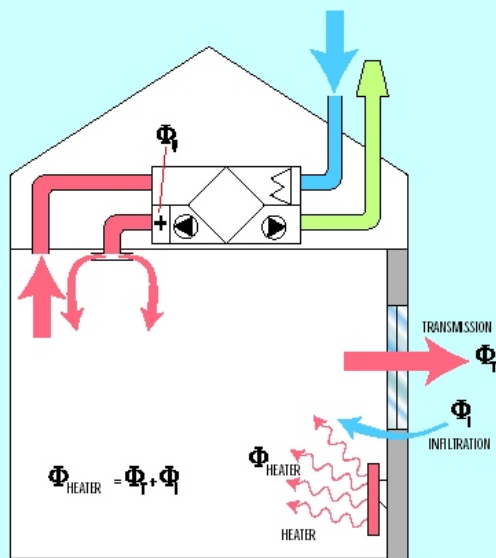
HEAT LOSS DUE TO BALANCED VENTILATION
