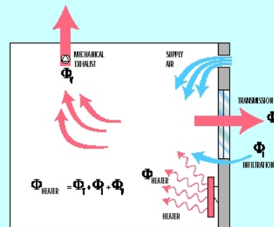
HEAT LOSS DUE TO MECHANICAL EXHAUST VENTILATION
