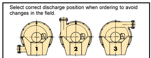
Standard discharge positions (viewed from motor side).
